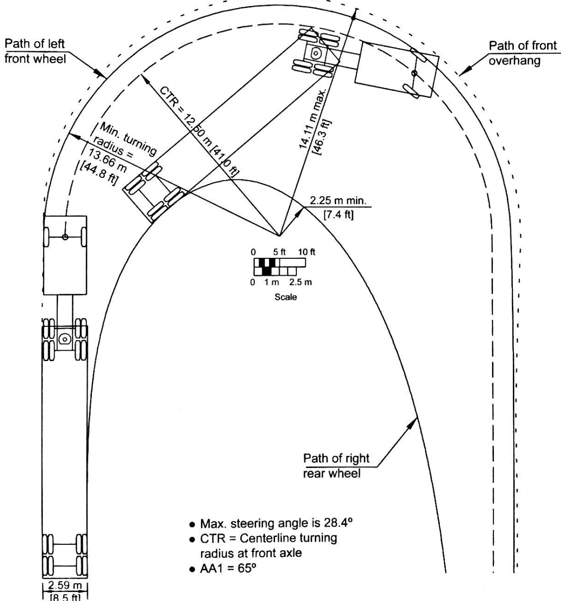
Figure 2-14. Minimum Turning Path for Interstate Semitrailer (WB-19 [WB-62]) Design Vehicle
